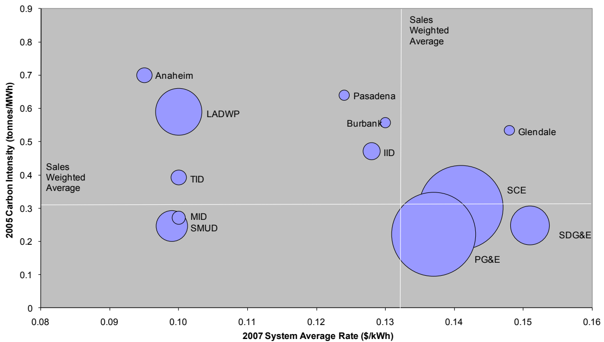
Carbon Intensity versus Average Retail Rate Ten Largest Local Distribution Companies (Bubble Size shows 2007 GWh Sales)
